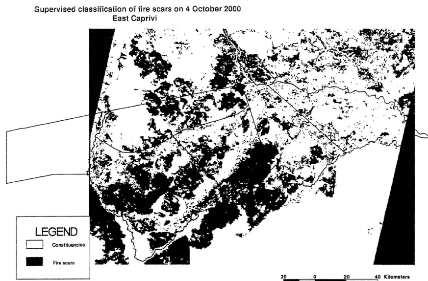
Figure 3. Supervised Classification (Maximum Likelihood procedure) of bands 3,4,5, and 7 of Landsat TM image (path 174 rows 072–073) dating of 4 October 2000. The straight vertical boundary between a large burned area and an unaffected area in the lower left portion is a wide annually maintained firebreak in Botswana.
